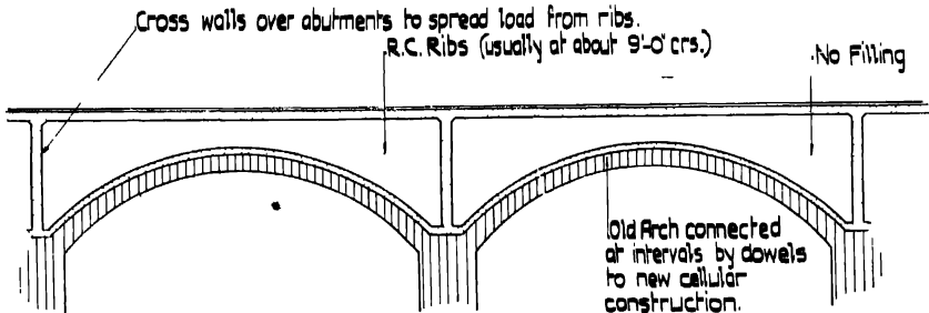
Fig. 214.—Relieving Old Arches from all Loads by New Reinforced Concrete Cellular Construction.
